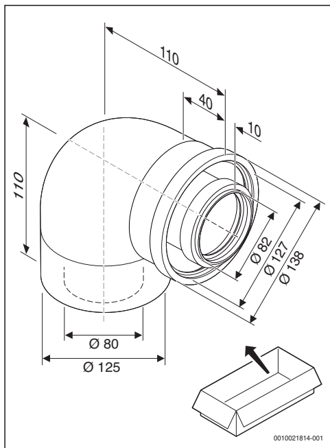
2 FC-CE80-87
